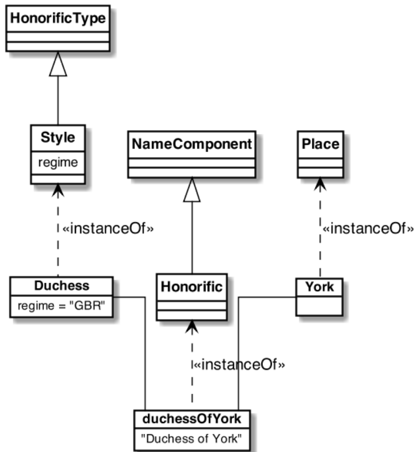
Figure 11 – An example of names with honorific presented in terms of class instantiations.
