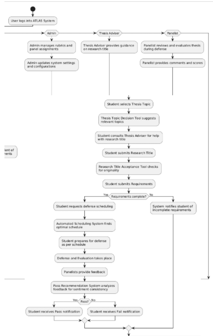
Figure 10. Activity Diagram
