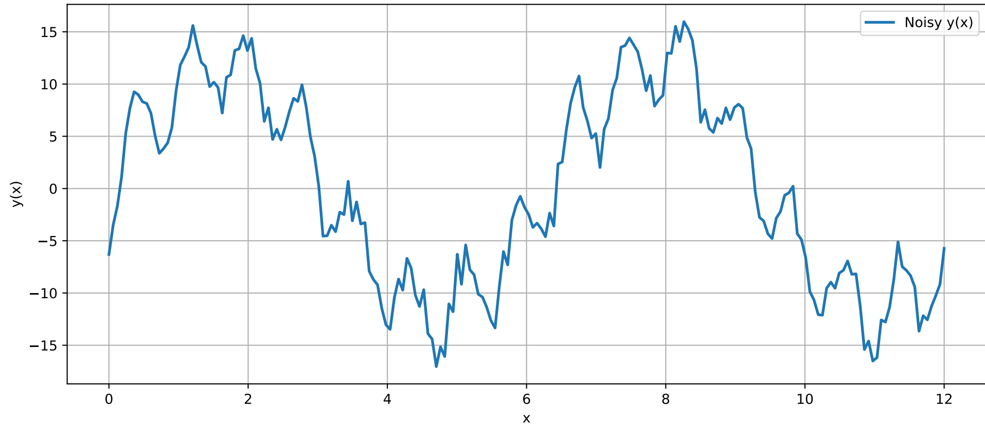
(b) Noisy Signal: y(x) = 12\sin(x) - 4\cos(8x)
