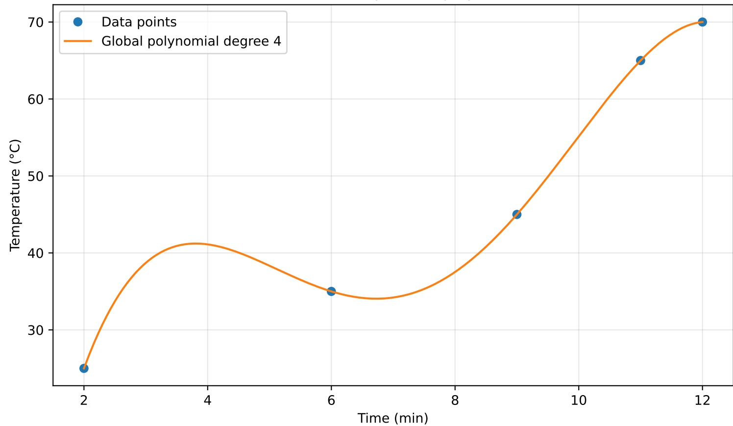
(c) Global interpolation polynomial
