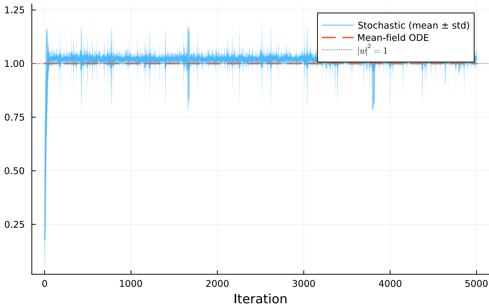
Norm dynamics, \eta = 0.03 , \rho = 0.9
