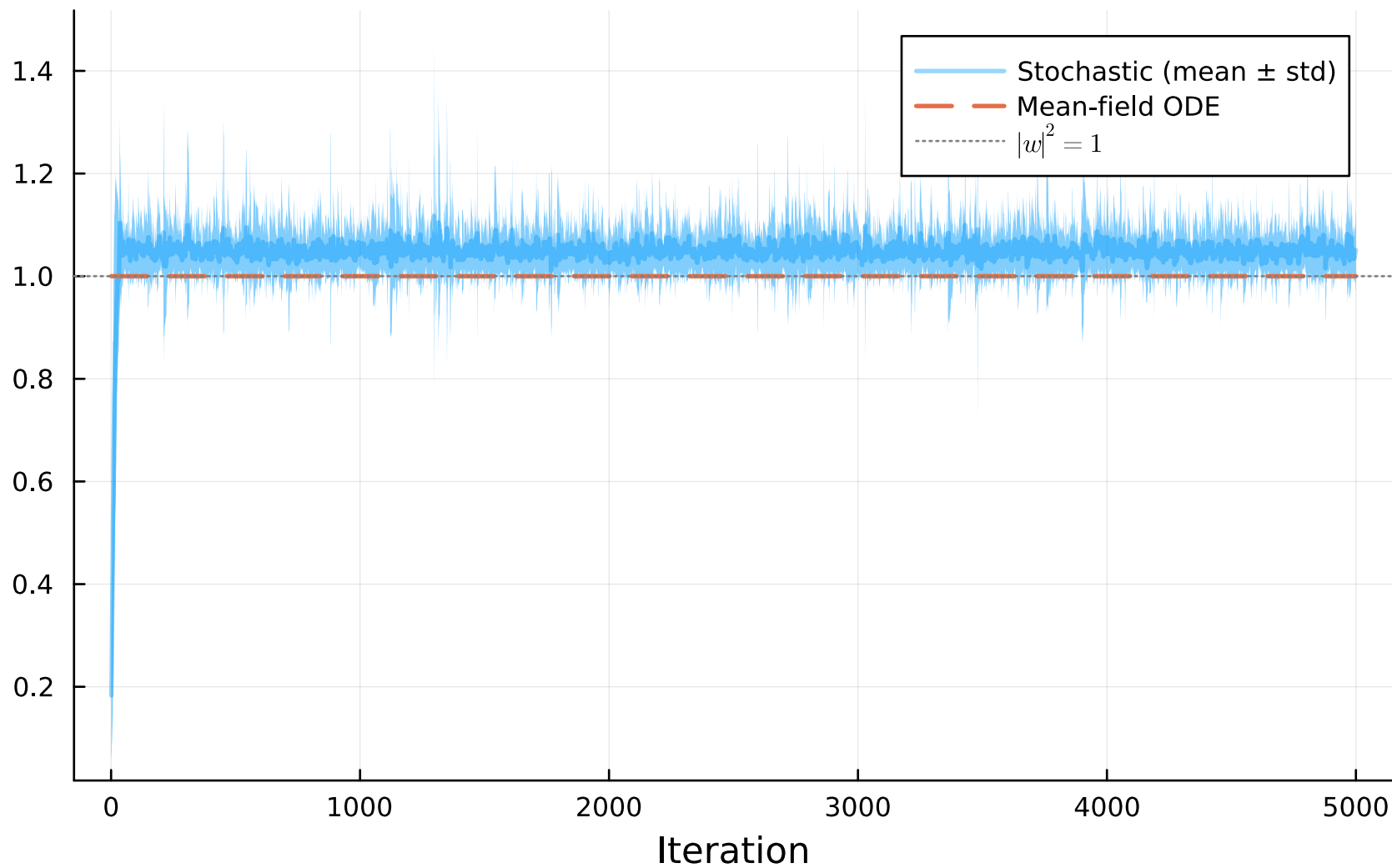
Norm dynamics, \eta = 0.03 , \rho = 0.0
