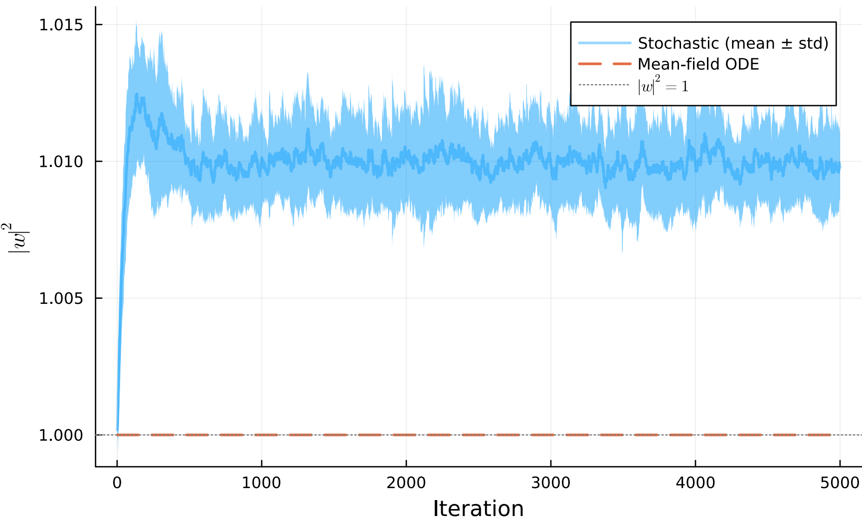
Norm dynamics, \eta = 0.003 , \rho = 0.0
