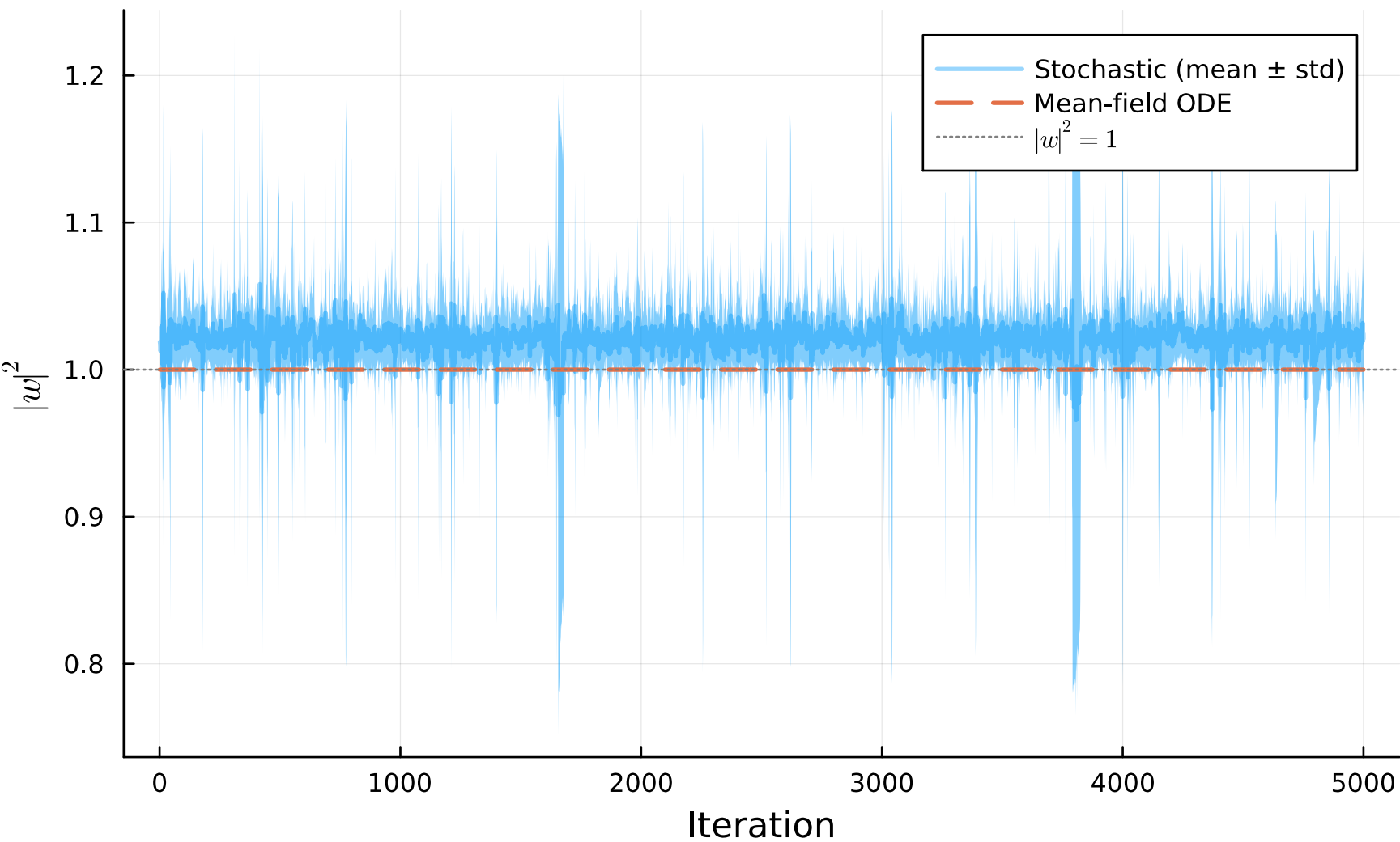
Norm dynamics, \eta = 0.03 , \rho = 0.9
