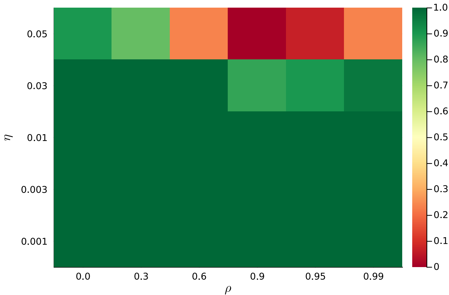
Fraction of non?—divergent runs
