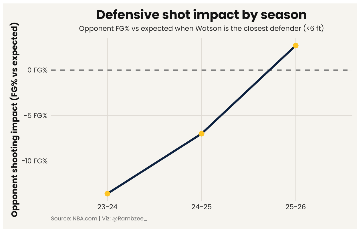
Figure 4: Opponent FG% impact by season (Diff%). Negative is better if Diff% means DFG% minus expected FG%.
