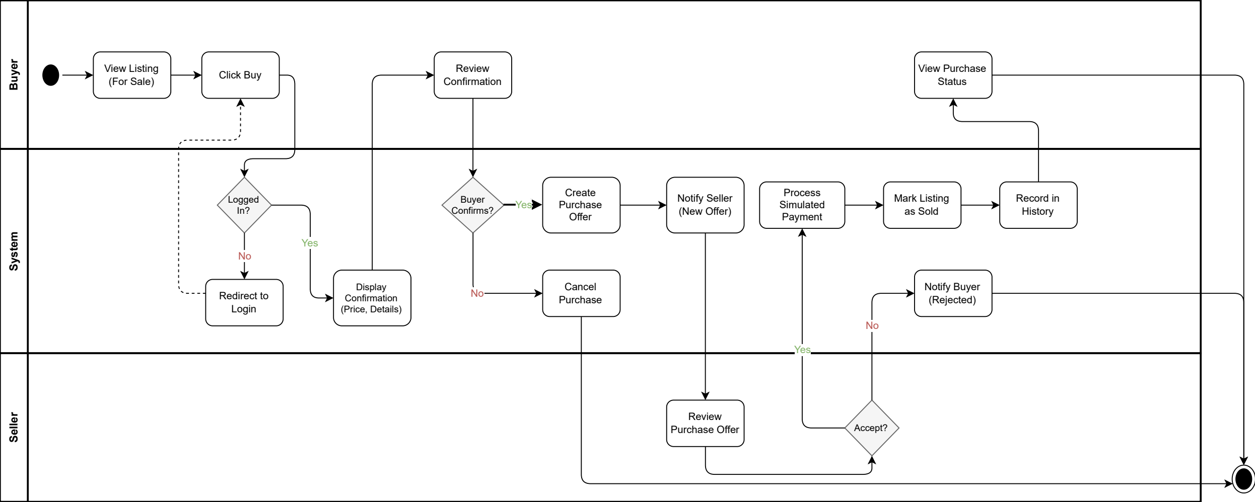
US-10: Purchase Item - Activity Diagram
