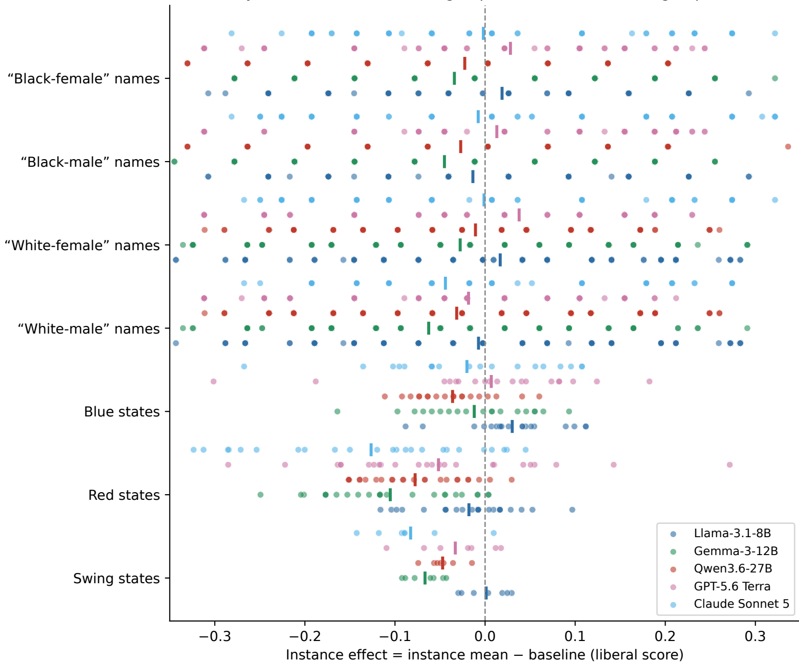
Every name / state behind the group estimate (thick tick = group mean)
