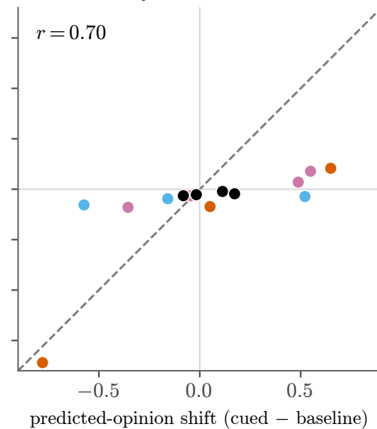
Qwen-3.6-27B
