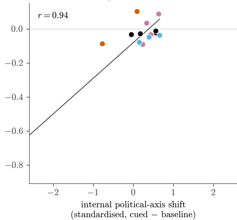
Qwen-3.6-27B
