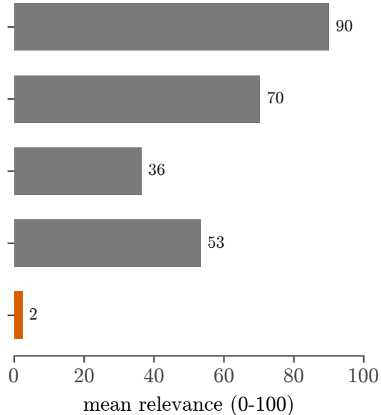
Qwen-3.6-27B
