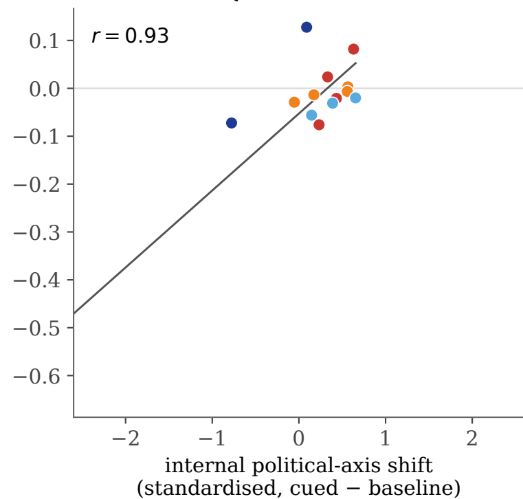
Qwen3.6-27B
