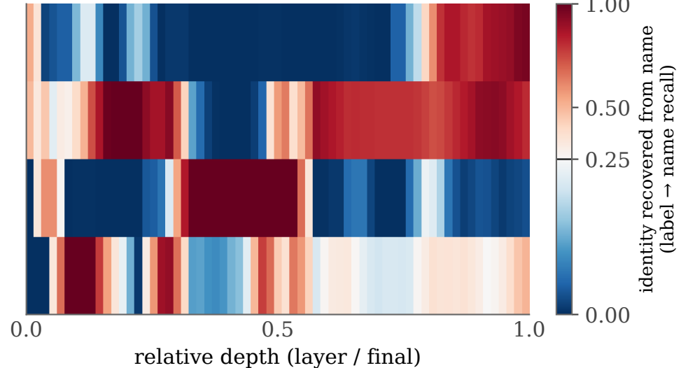
Qwen3.6-27B
