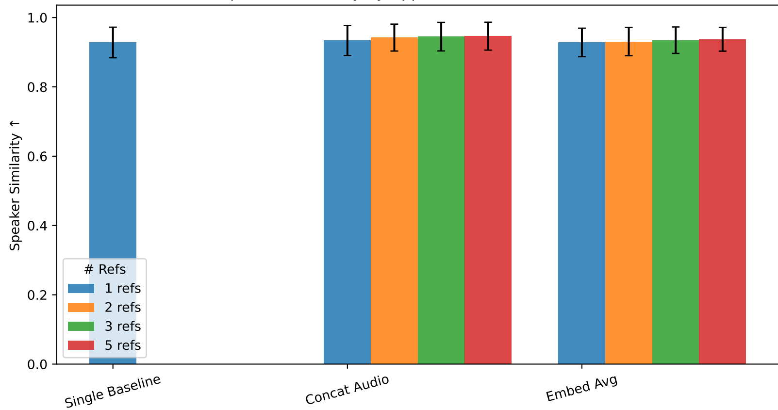
Speaker Similarity by Approach × Num References
