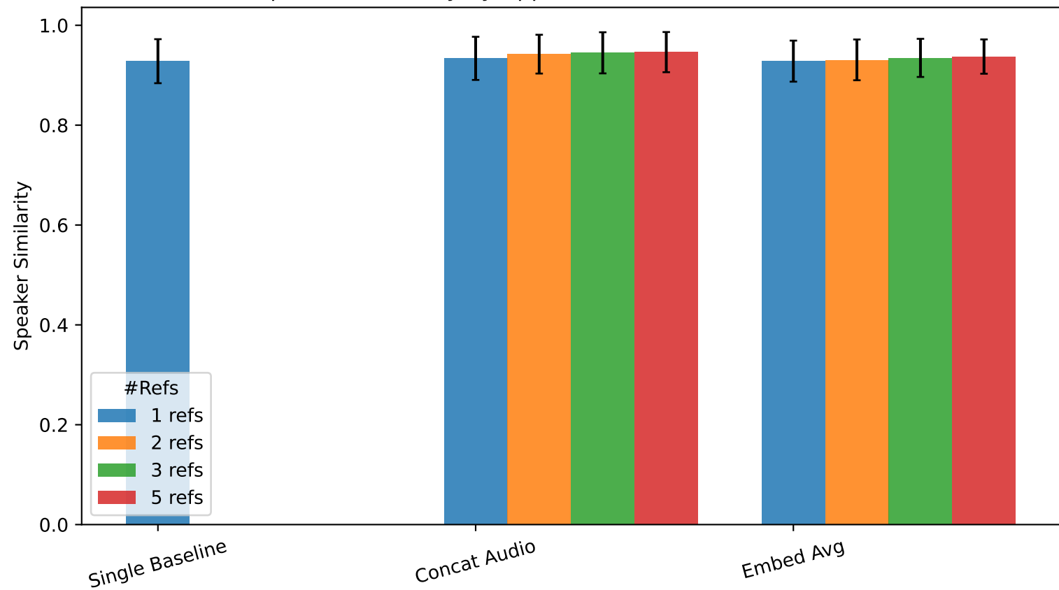
Speaker Similarity by Approach x Number of References
