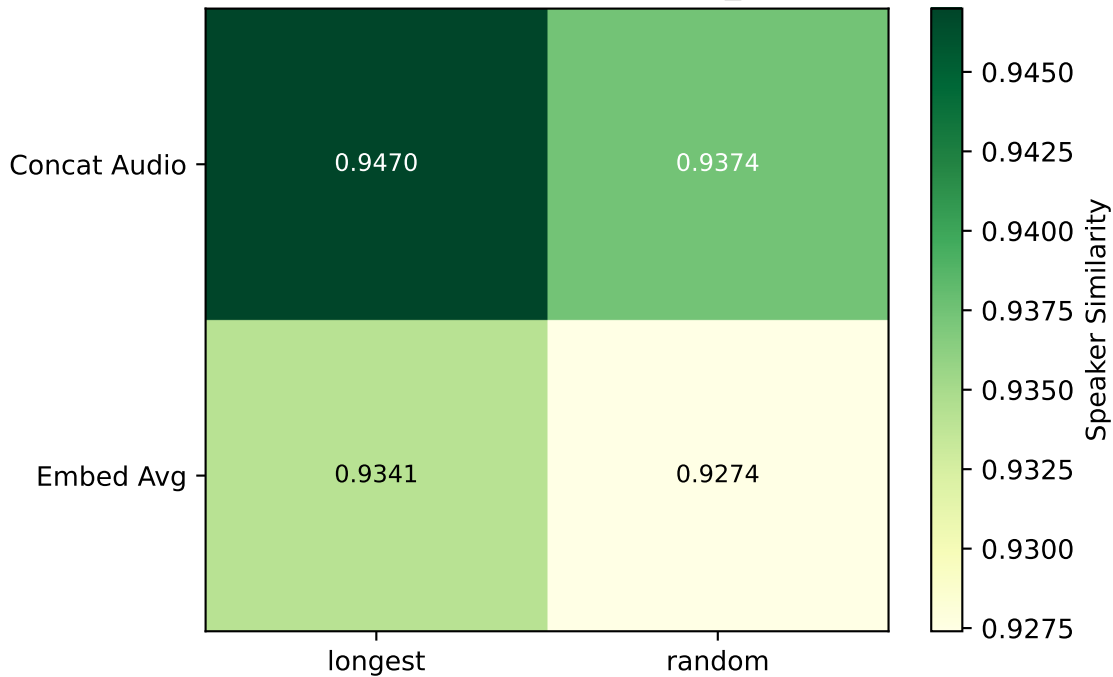
Speaker Similarity Heatmap (n_refs=2)
