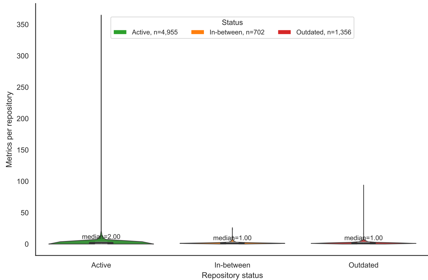
Metrics per repository by repository activity status
