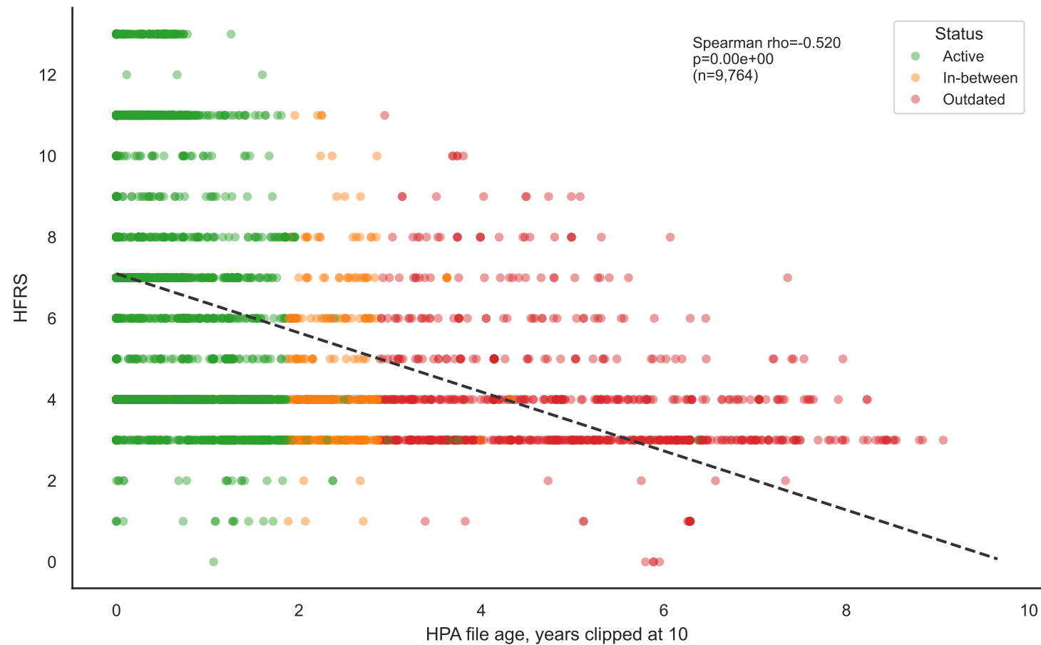
HFRS versus HPA file age
