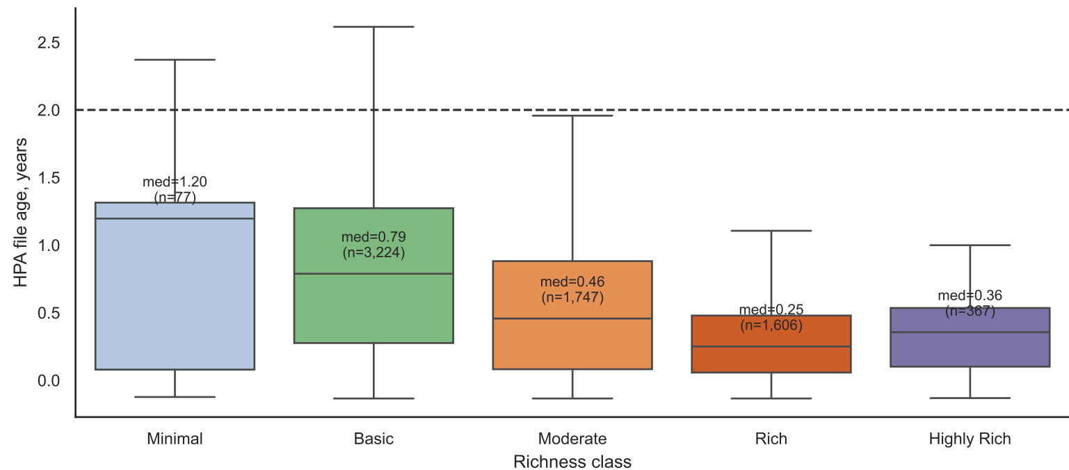
HPA file age by richness class in active repositories
