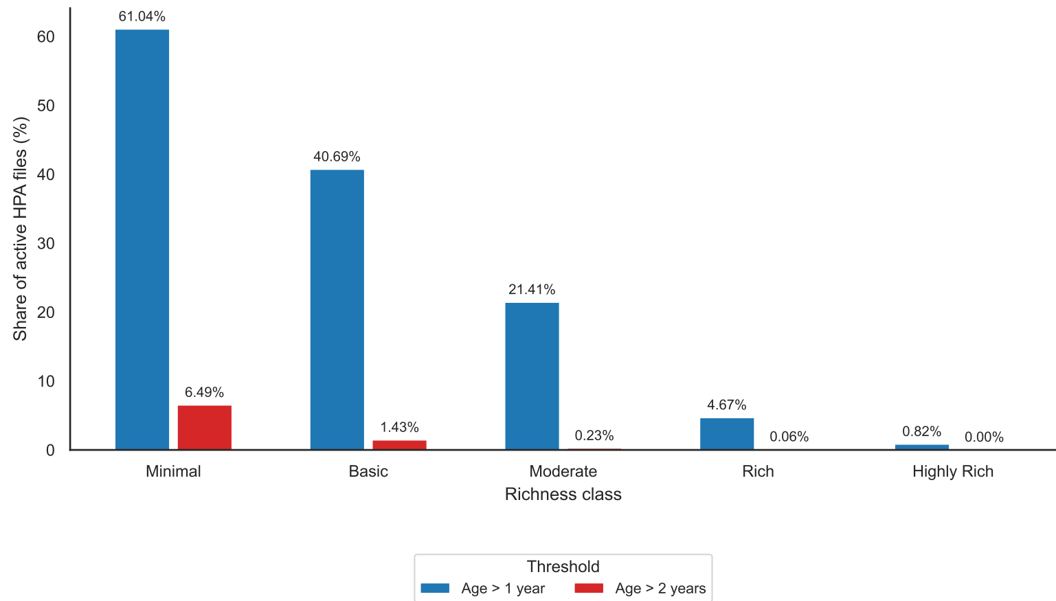
Older HPA files within active repositories
