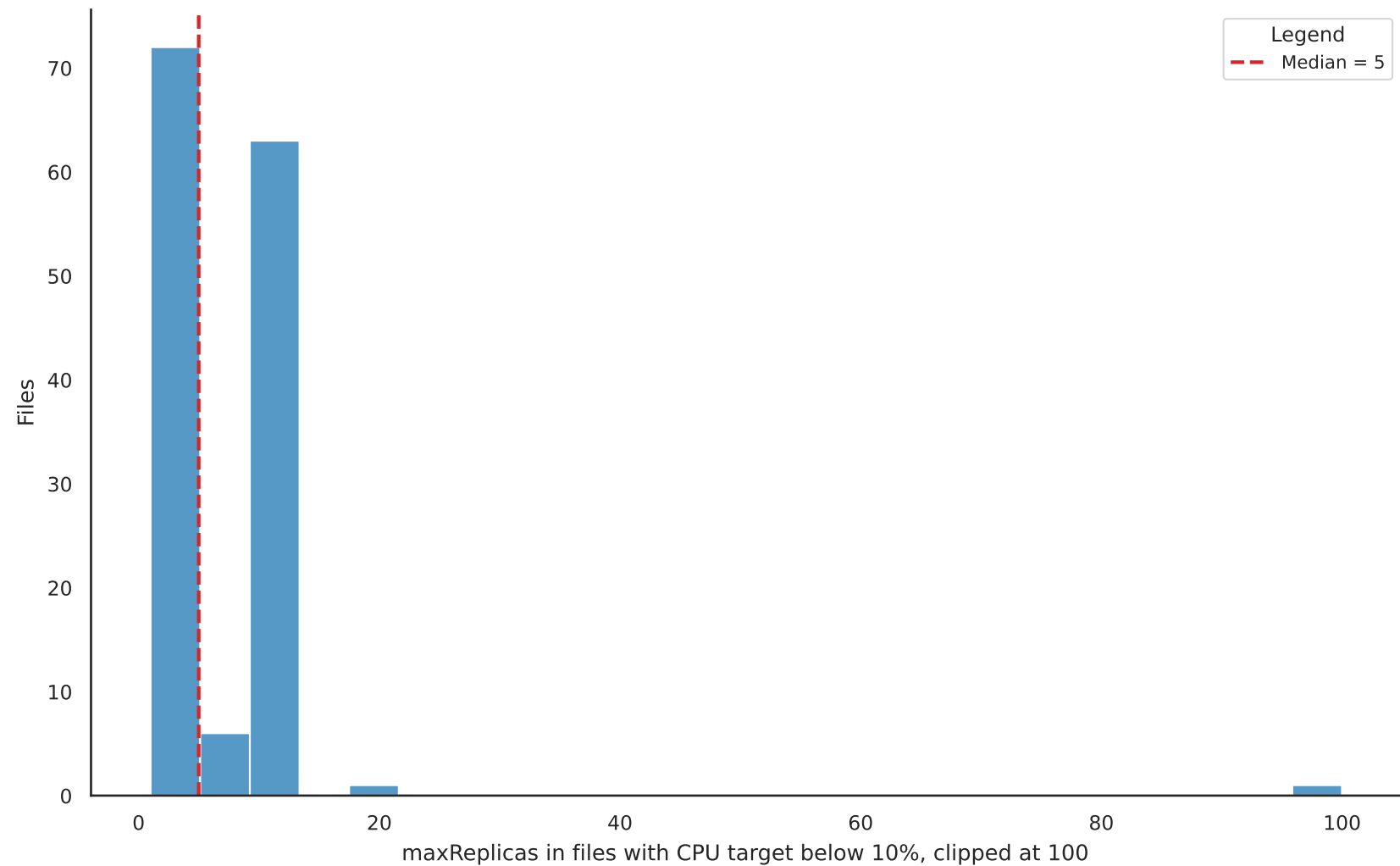
maxReplicas among low CPU-threshold files
