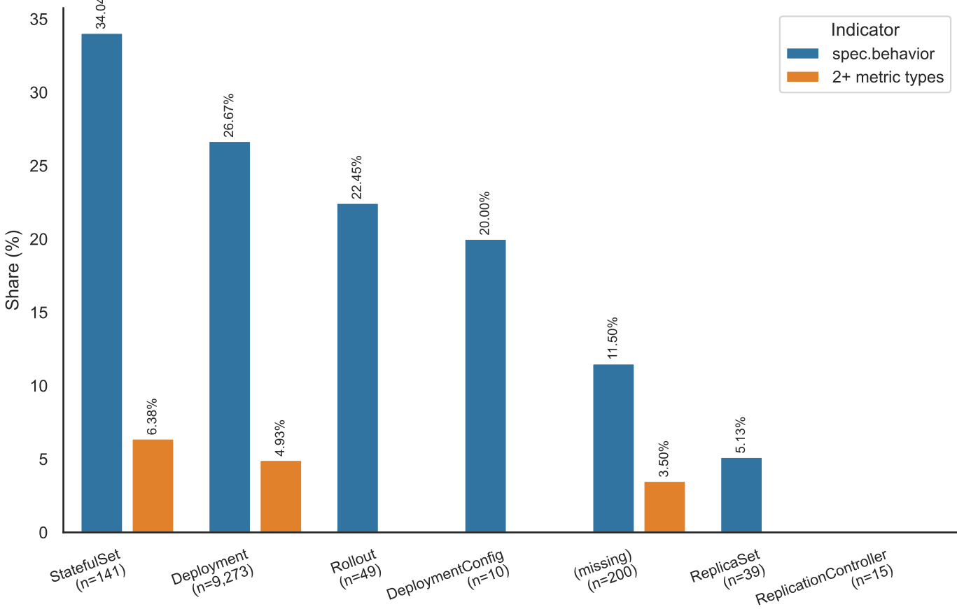
(B) spec.behavior and 2+ metric types by kind
