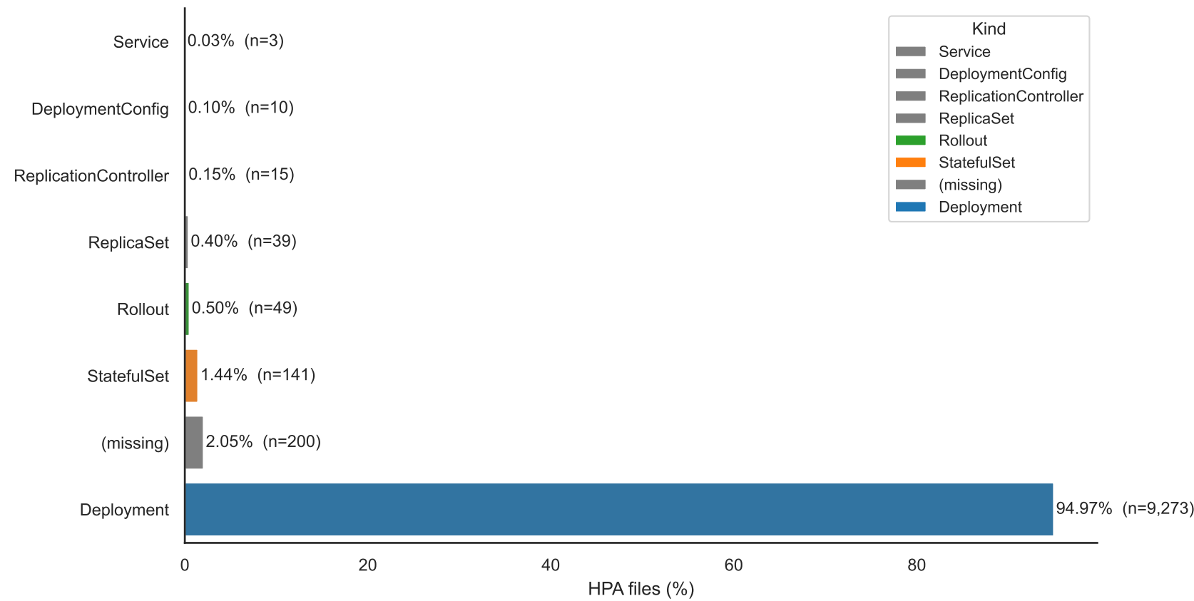
(A) Most common scaleTargetRef kinds
