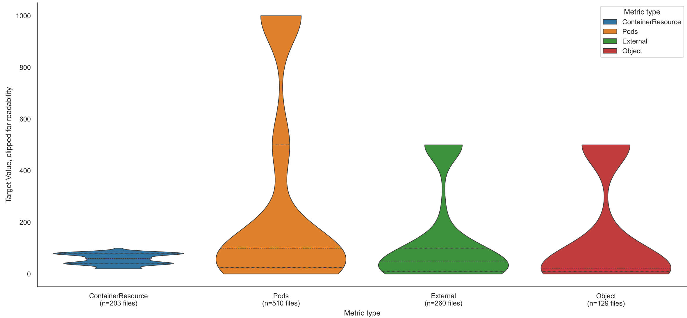
Target Value distribution for non-Resource metric types
