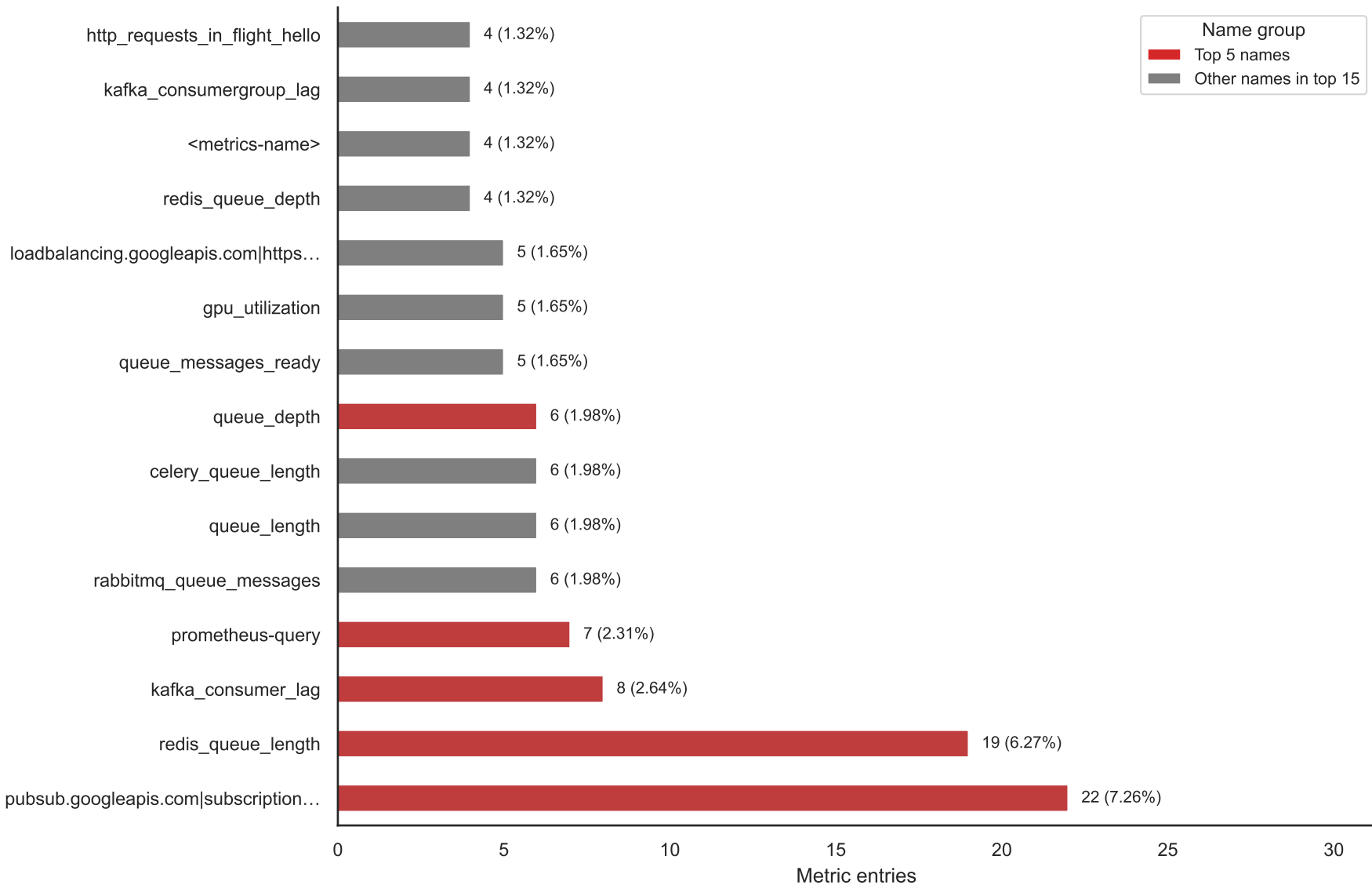
External metric names, long-tail distribution
