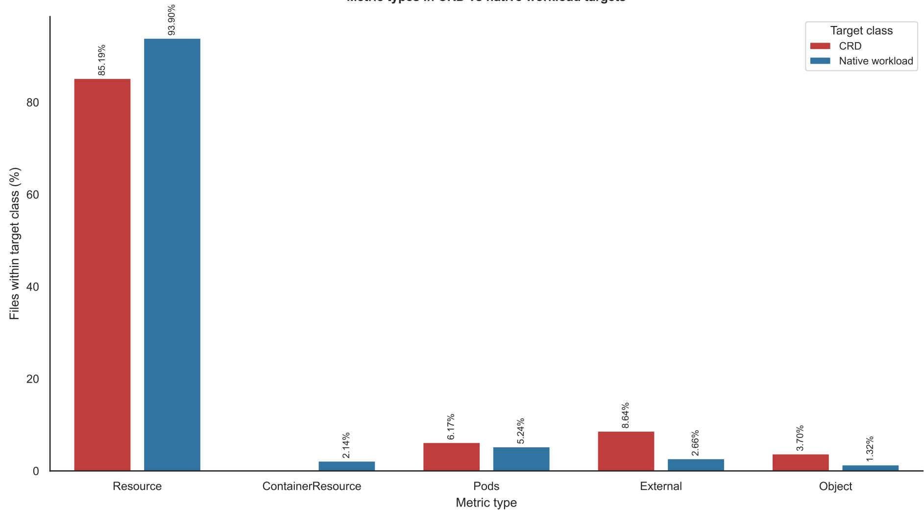
Metric types in CRD vs native workload targets
