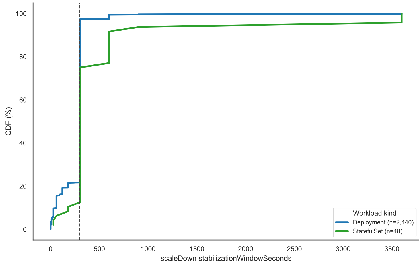
scaleDown stabilization, Deployment vs. StatefulSet
