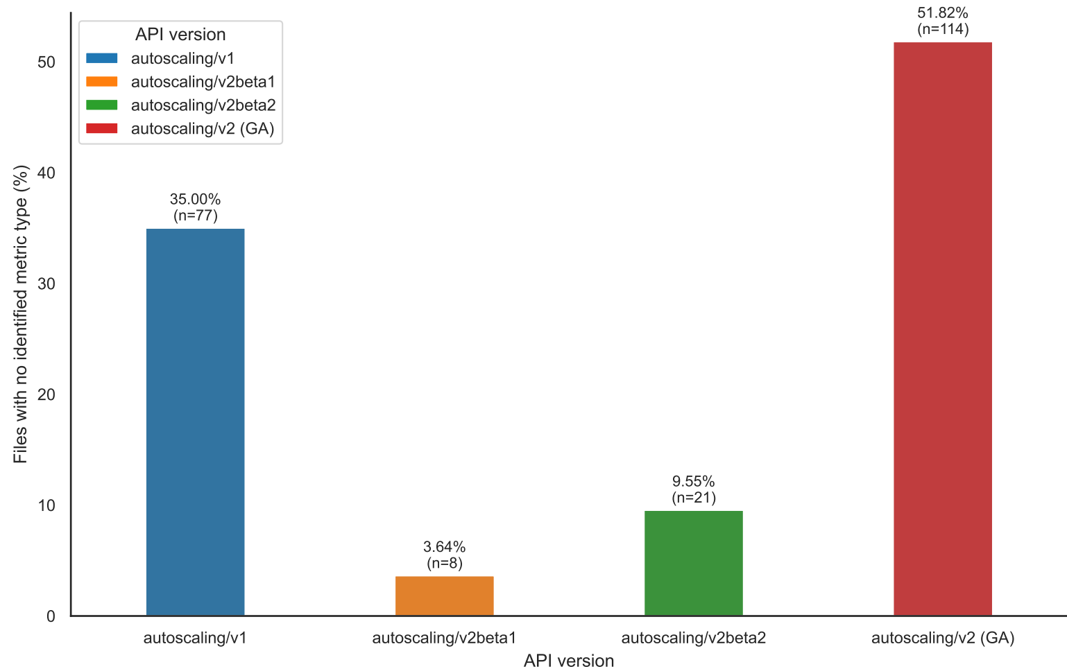
No-metric group by API version
