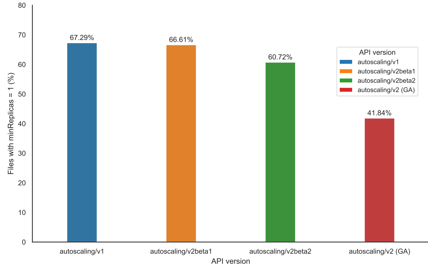
(B) Files with minReplicas = 1 by API version
