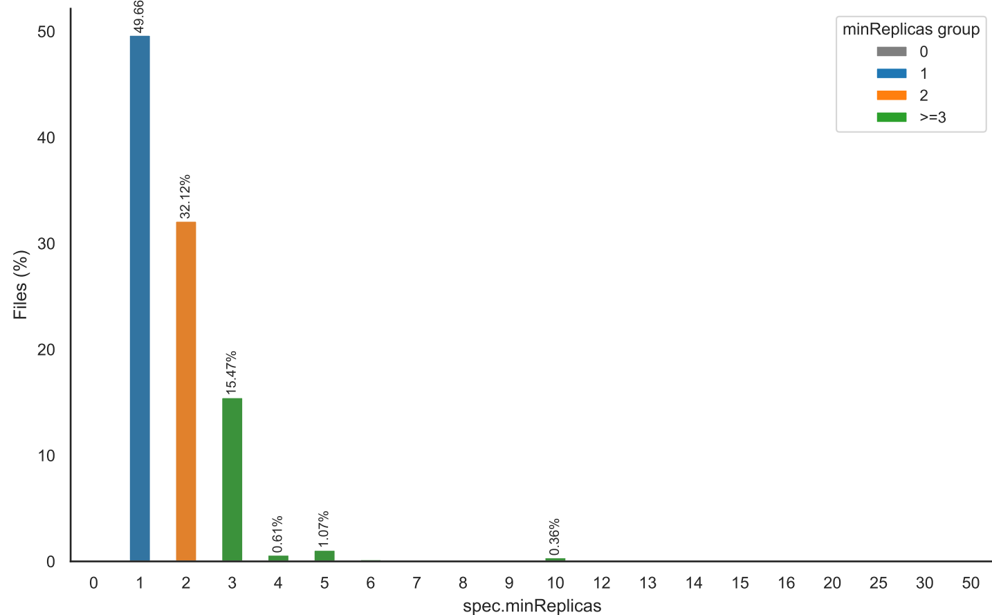
(A) Distribution of spec.minReplicas
