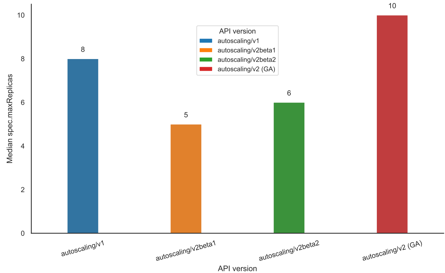
(B) Median maxReplicas by API version
