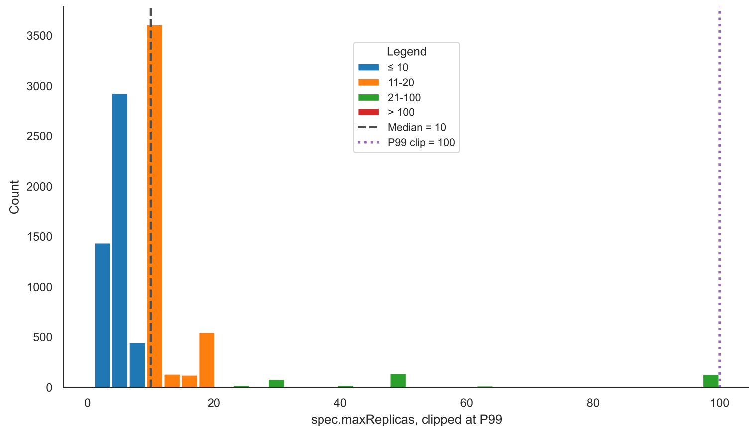
(A) Distribution of spec.maxReplicas
