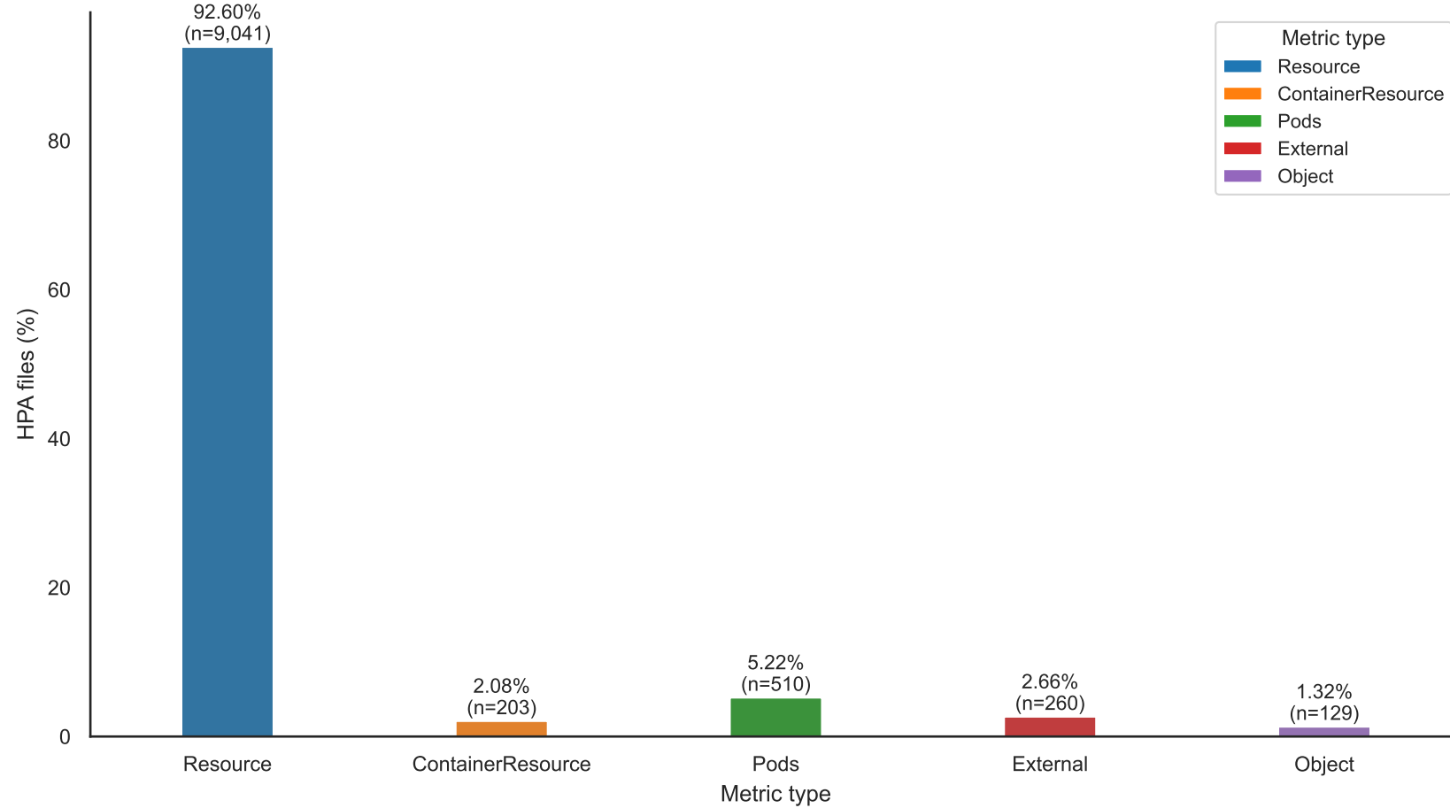
(A) Overall adoption of metric types
