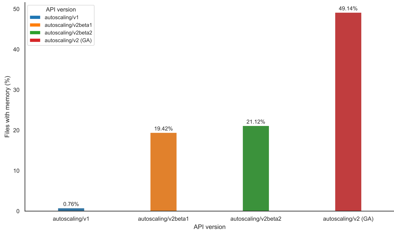
Memory adoption by API version
