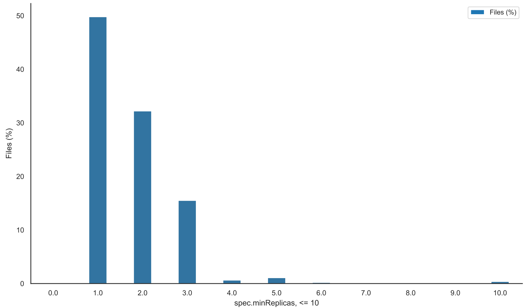
minReplicas distribution
