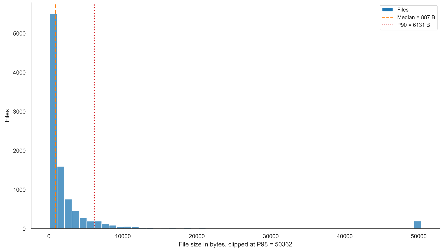
HPA file size distribution
