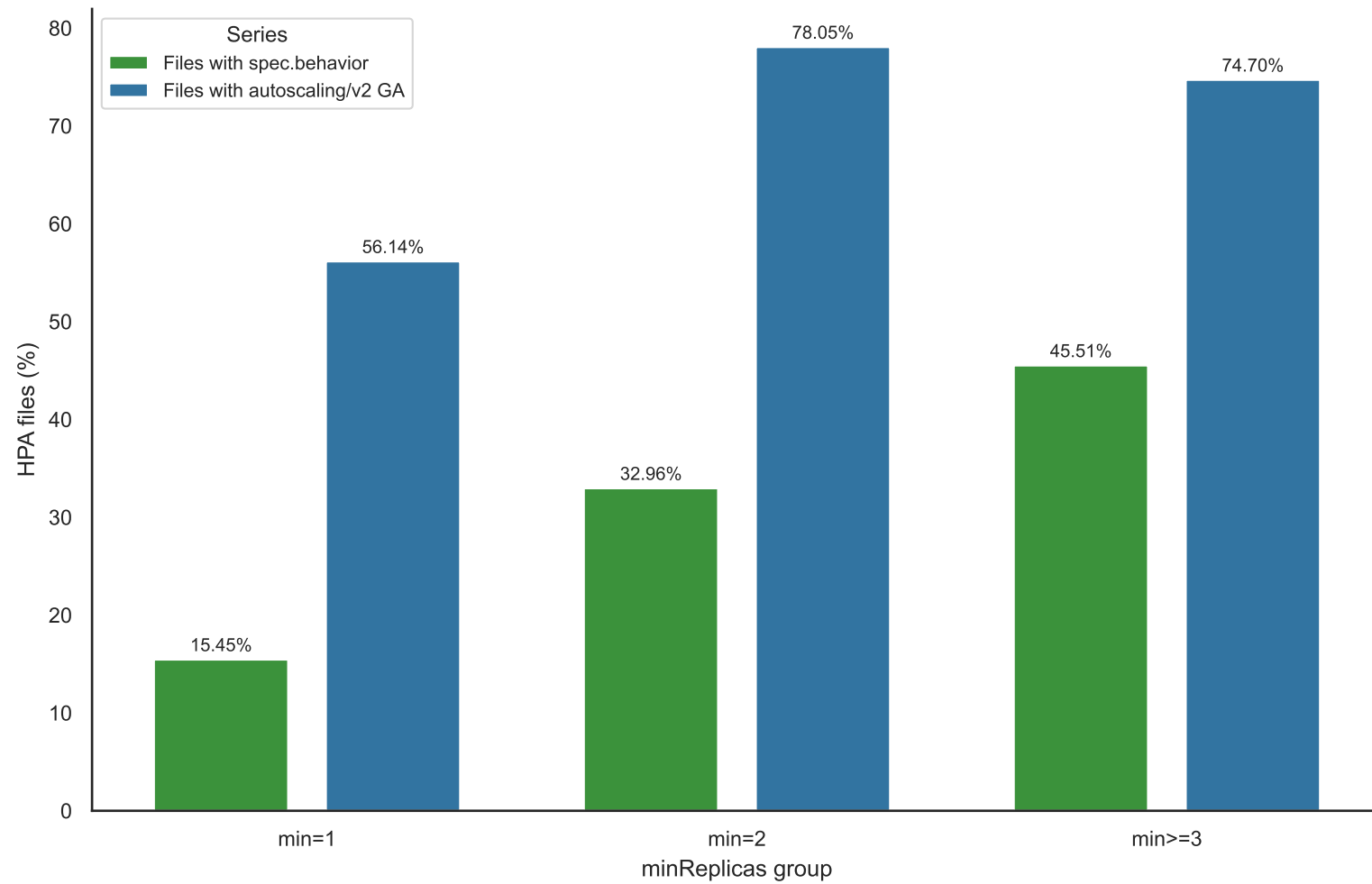
(A) behavior adoption and v2 usage by minReplicas
