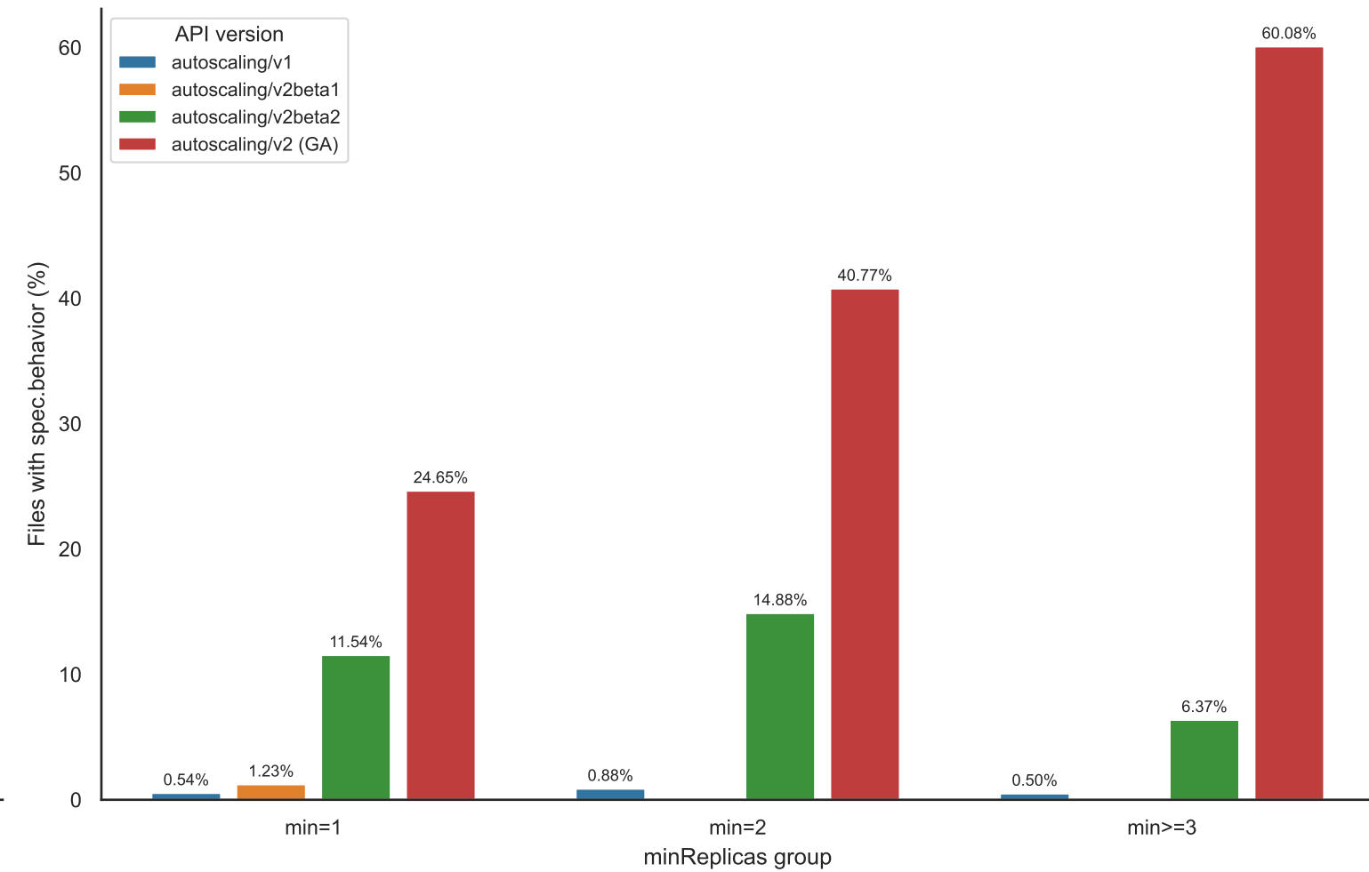
(B) behavior adoption by minReplicas and API version
