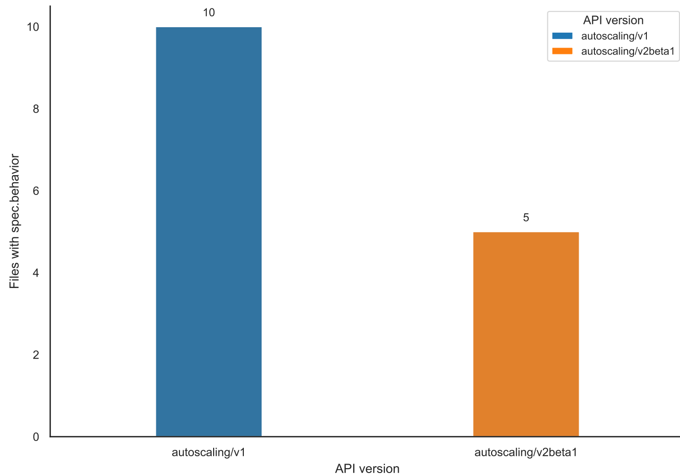
(A) Incompatible API versions
