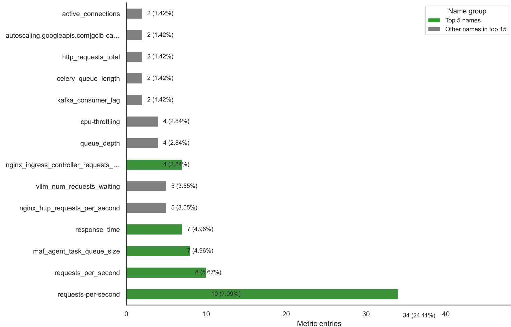
Object metric names, long-tail distribution
