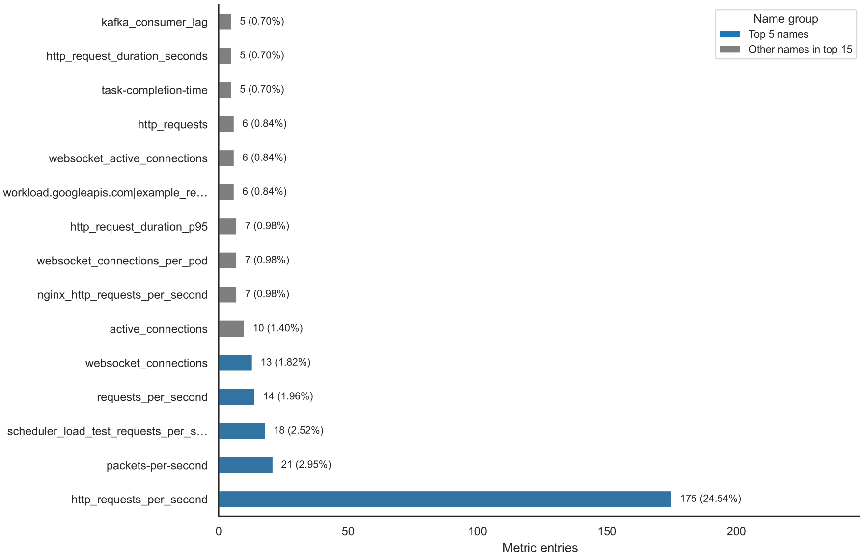
Pods metric names, long-tail distribution
