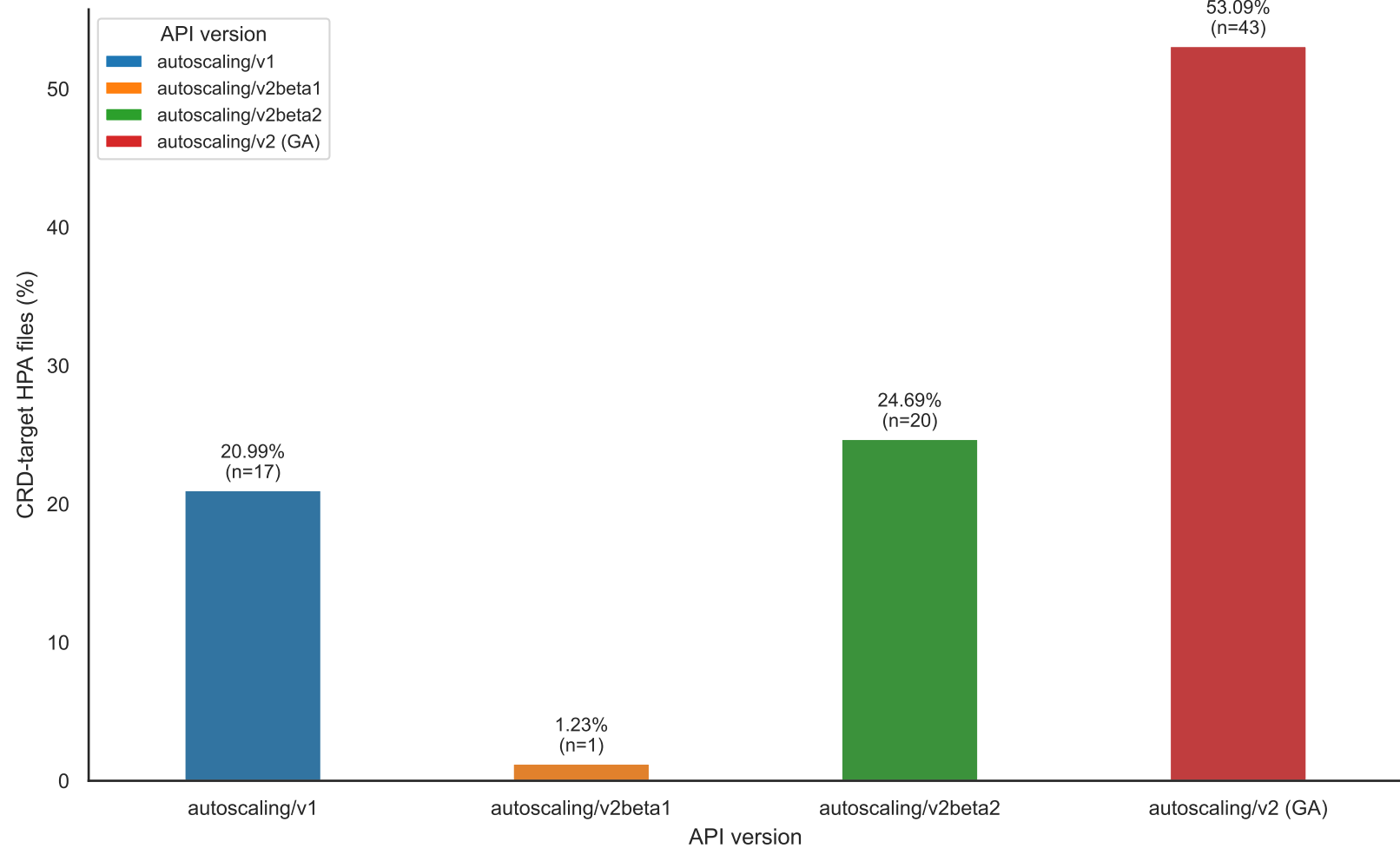
API version distribution among CRD targets
