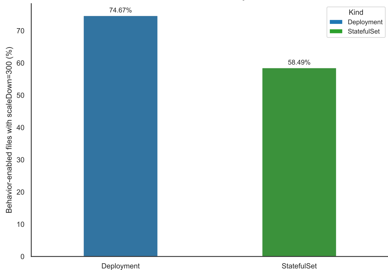
Default scaleDown stabilization by workload kind
