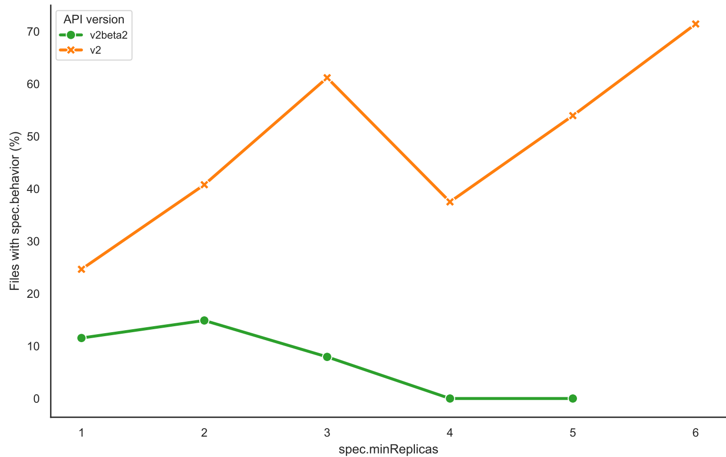
spec.behavior by minReplicas and API version
