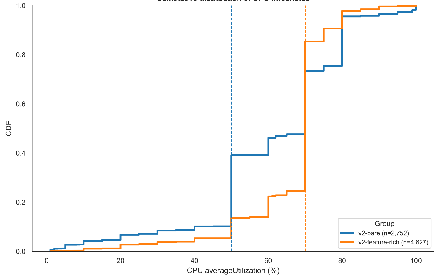
Cumulative distribution of CPU thresholds
