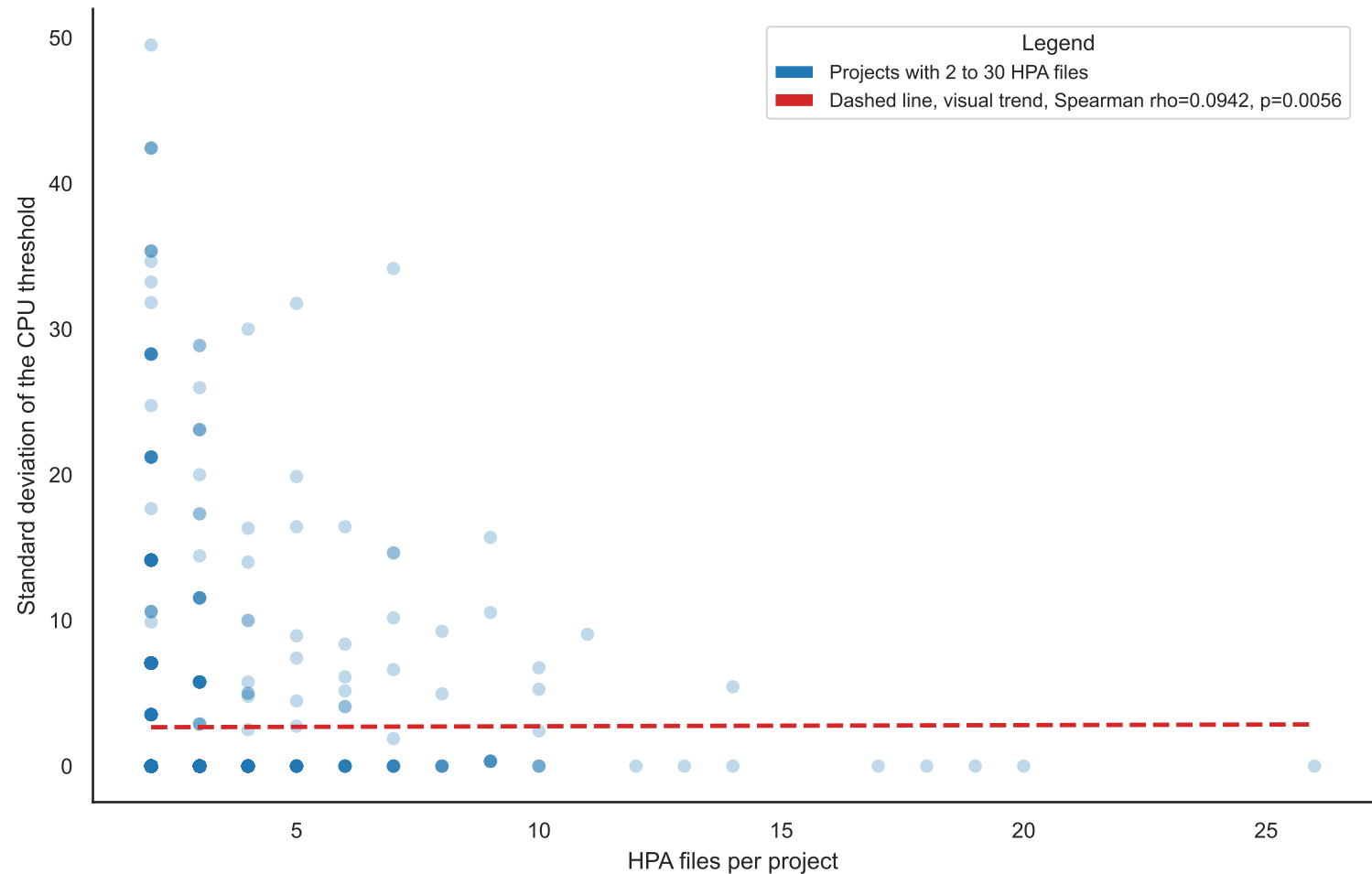
Project size vs. CPU-threshold dispersion
