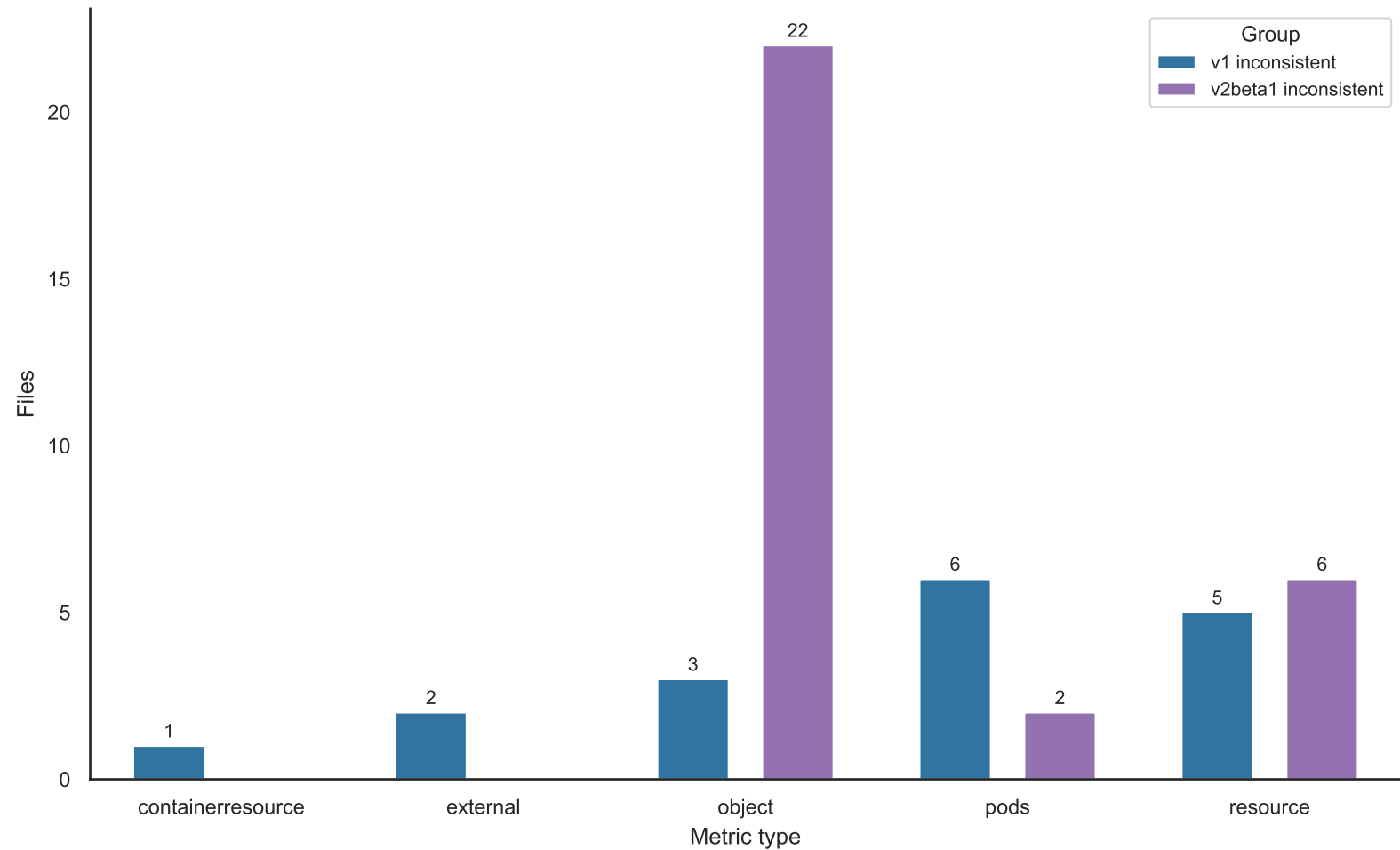
Metric types found in inconsistent version/type cases
