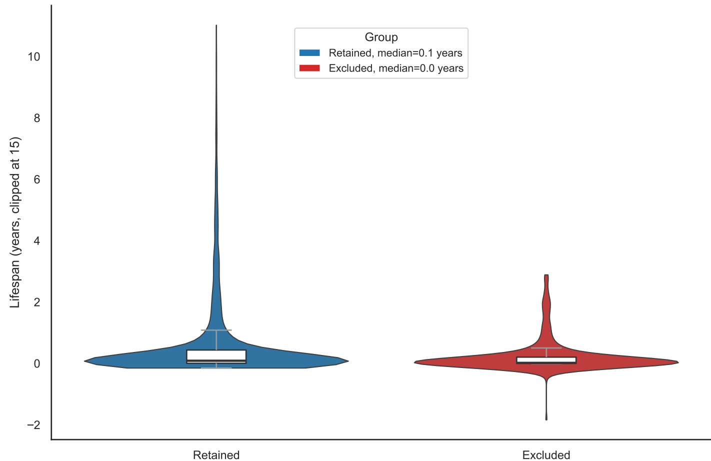
Repository lifespan: retained vs. excluded repositories
