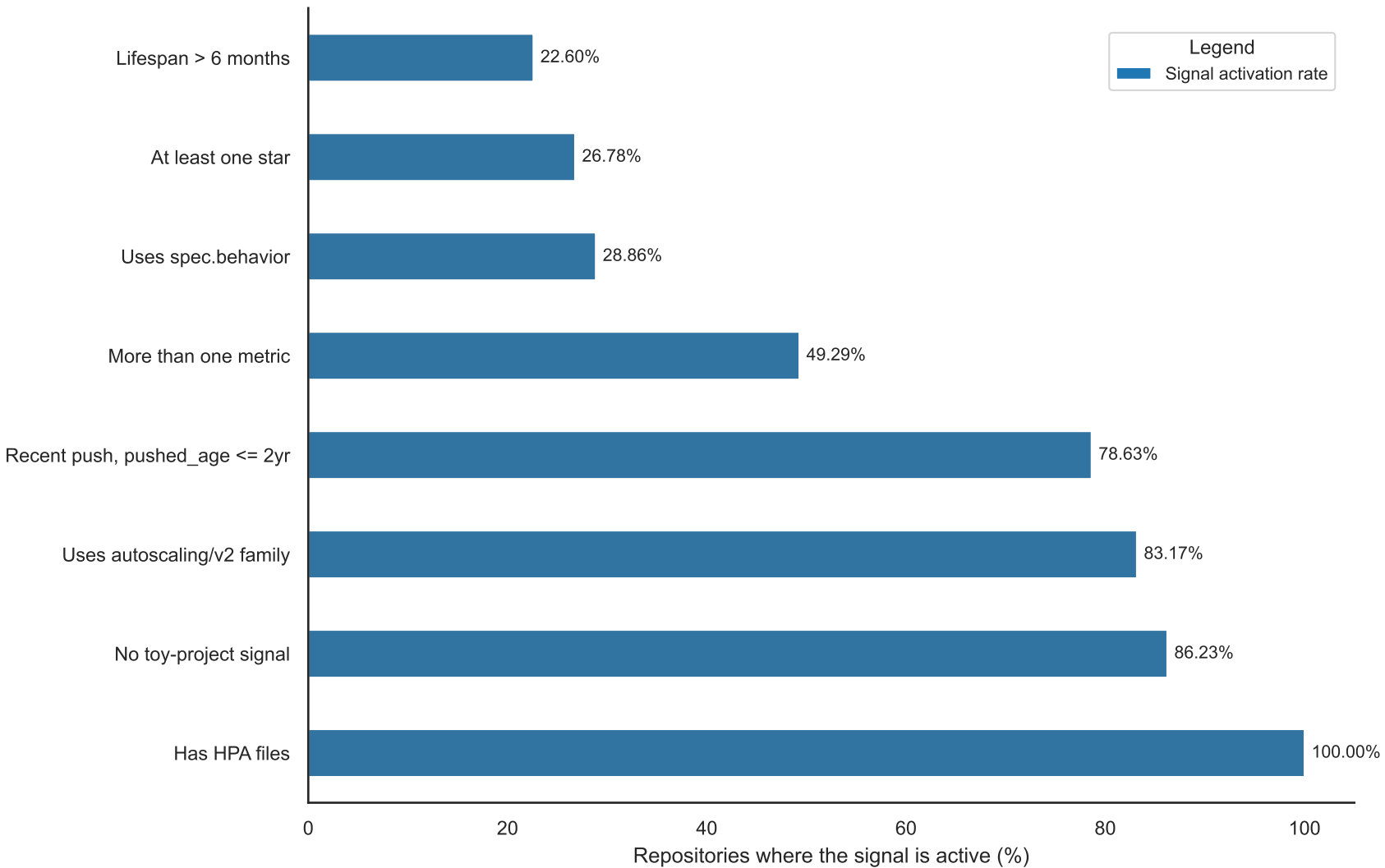
Activation rate of each confidence-score signal
