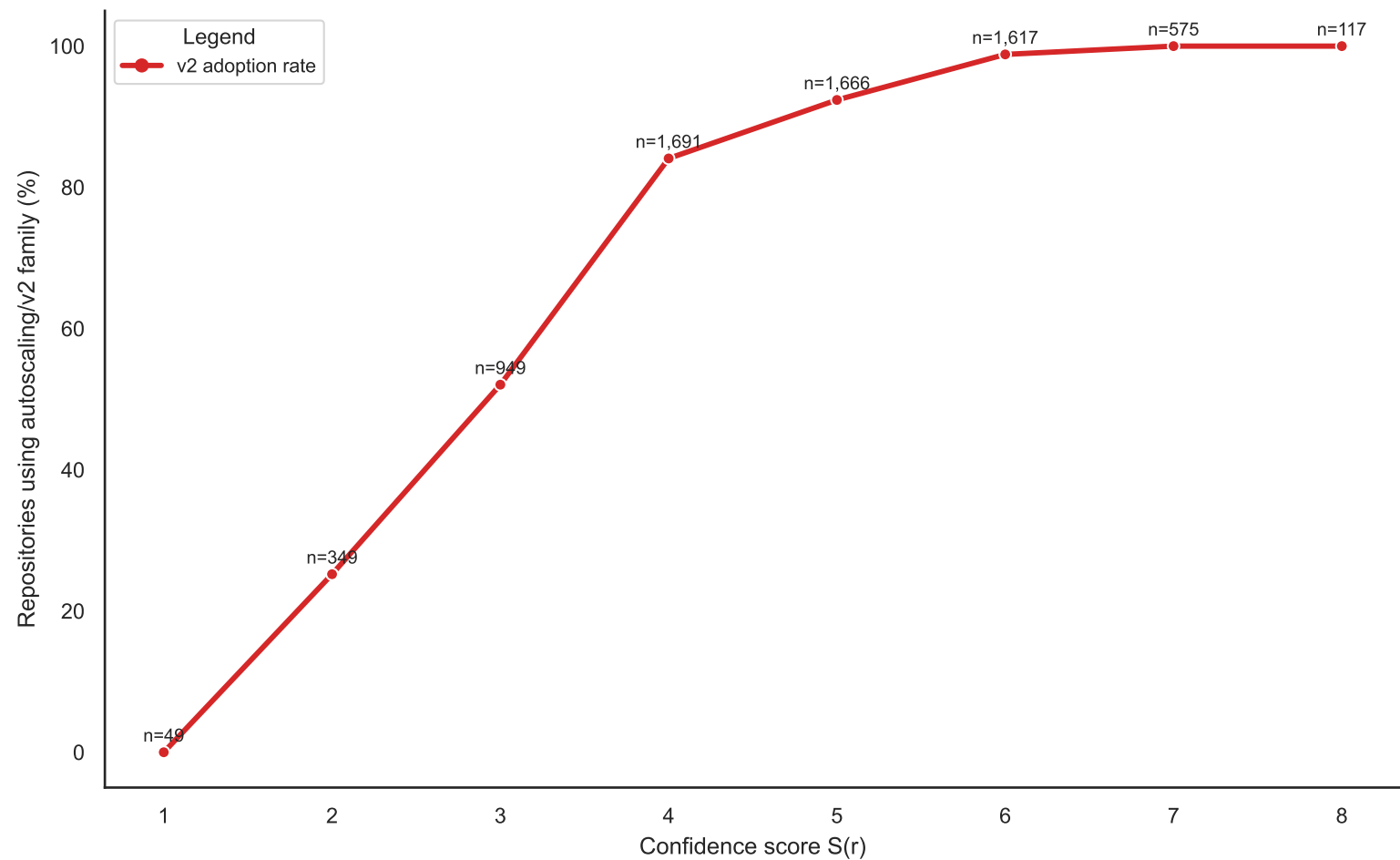
autoscaling/v2 adoption by confidence-score level
